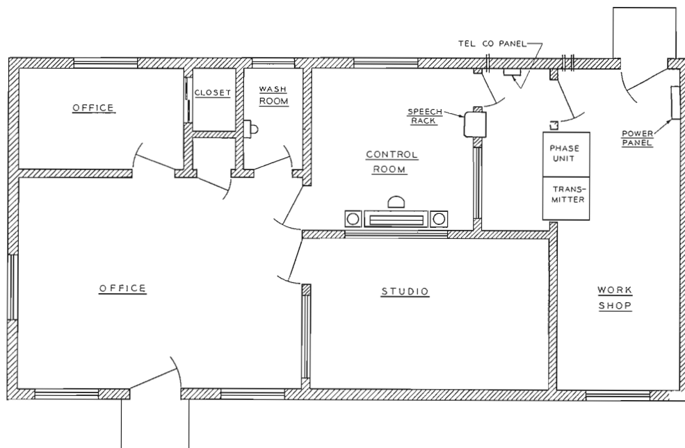
Floor plan of the WEBB combined studio-transmitter.
