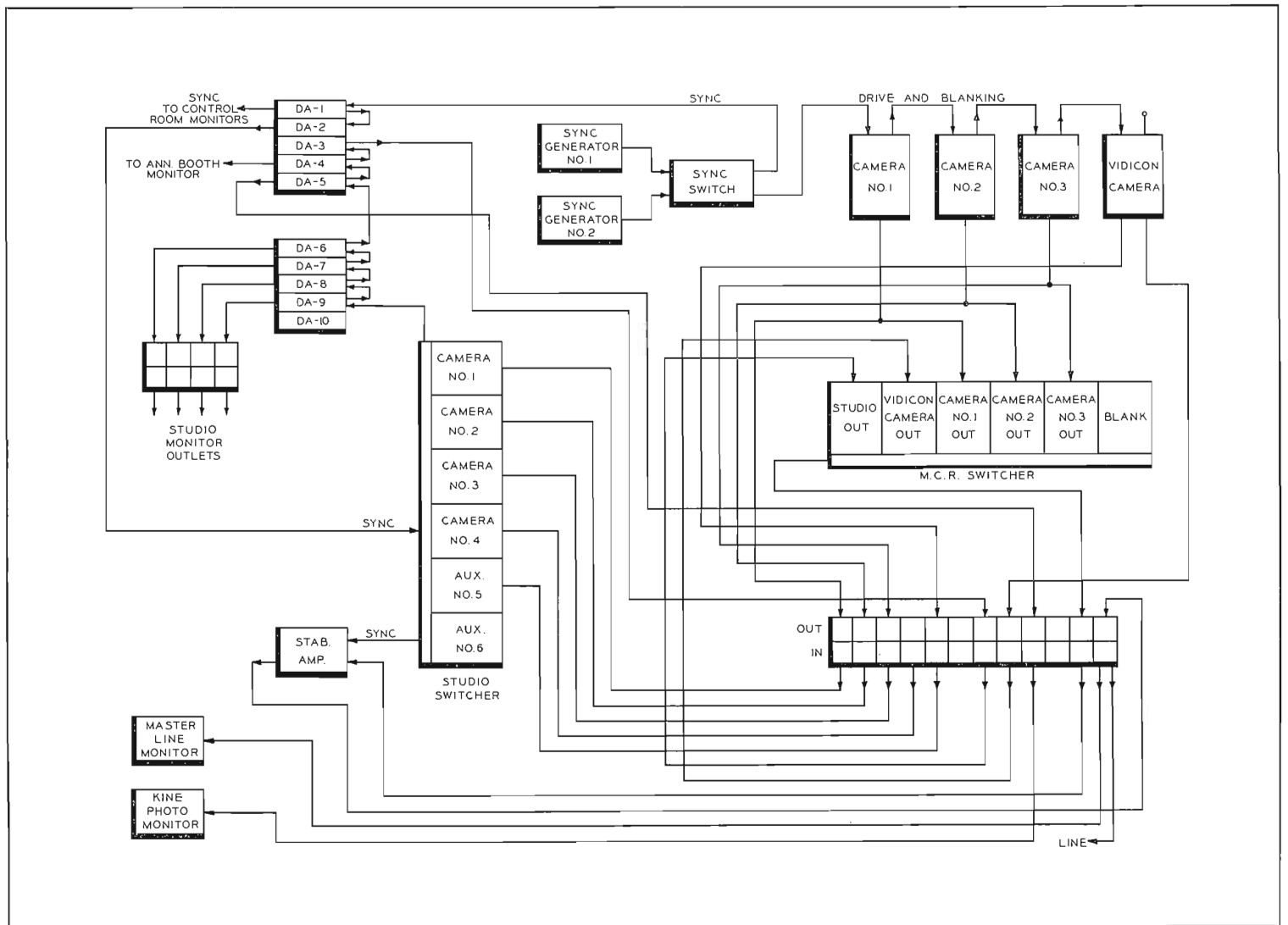
Video distribution diagram of WQED studios.
