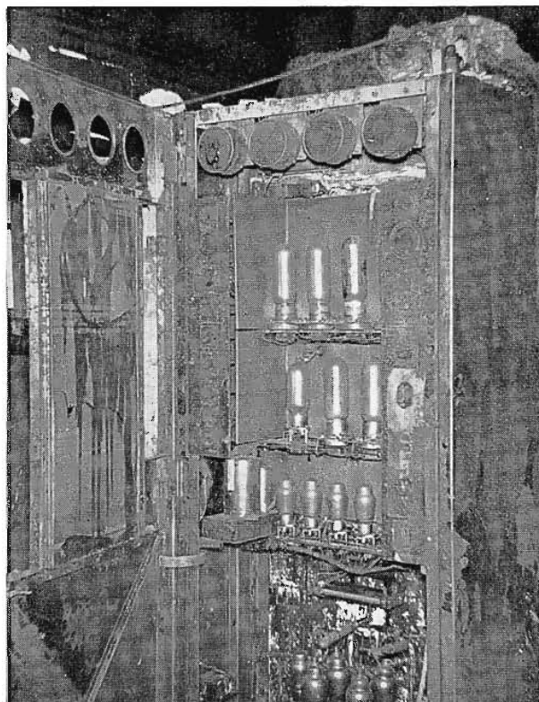
Fire-damaged equipment at WJPA. Replacement was made quickly with an RCA BTA-250M.
