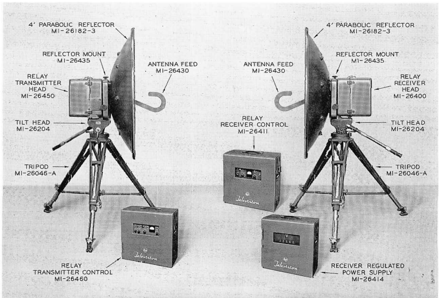
Equipment necessary for a single microwave link is shown below. A variety of mounting equipment is available for a multitude of applications.
