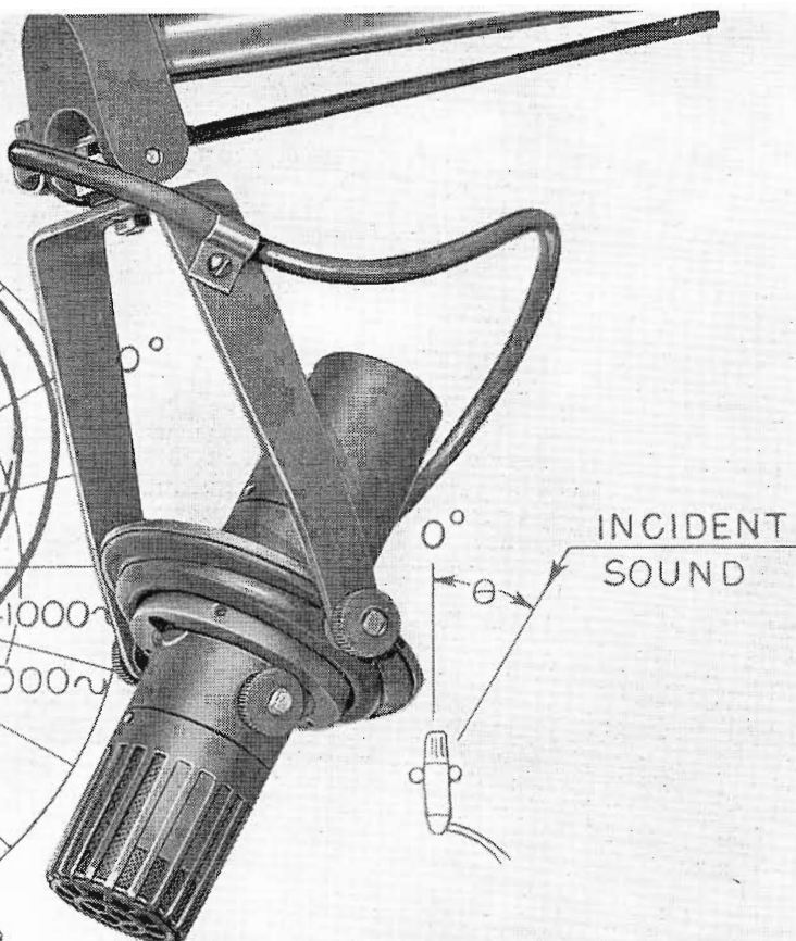
Directional characteristics of the BK-5A Microphone about the vertical axis.
